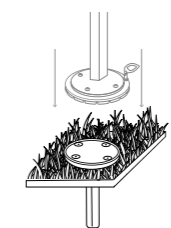
CONCRETE ANCHORAGE FOR ROTATION SUPPORT*
